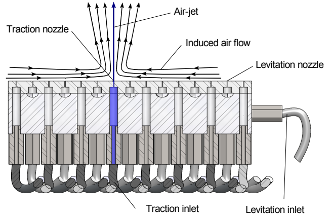
Fig. 2. Cross view of the induced air flow surface with one opened valve
